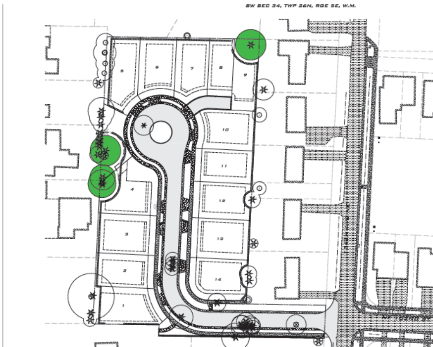
Tree Preservation Plan
