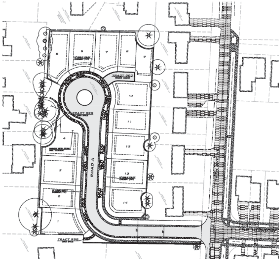
Site Plan
