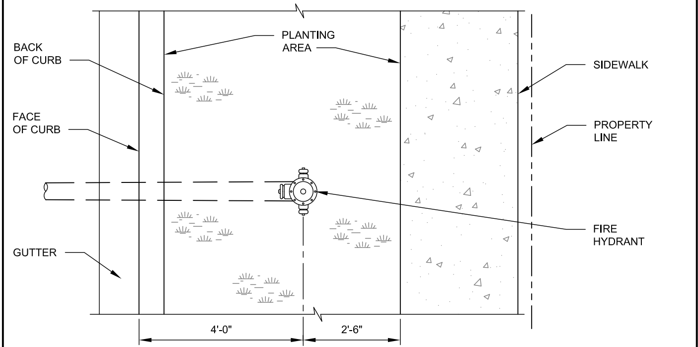
FIRE HYDRANT NTS
