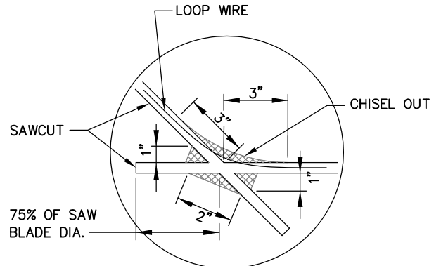
DETAIL B NTS
