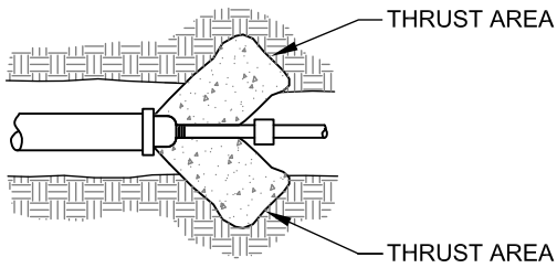
CAPS / PLUGS
